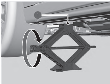
1 Jacking Point
