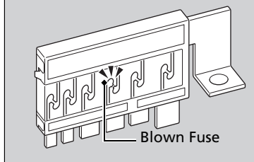
Combined Fuse
